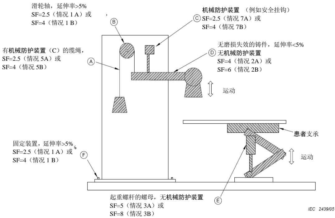
Figure A.17 – Example of determining Five-B safety factor using Table 21
